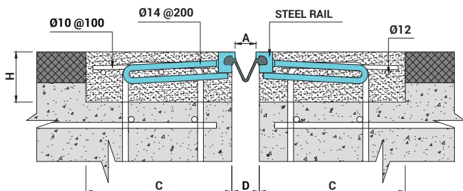
VHR-C STEEL STRIP-SEAL EXPANSION JOINT
