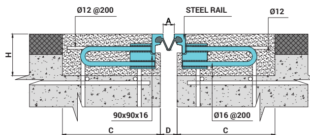
VHR-F80 (100) STEEL-STRIP SEAL EXPANSION JOINT
