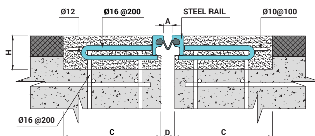
VHR-F50 STEEL STRIP-SEAL EXPANSION JOINT
